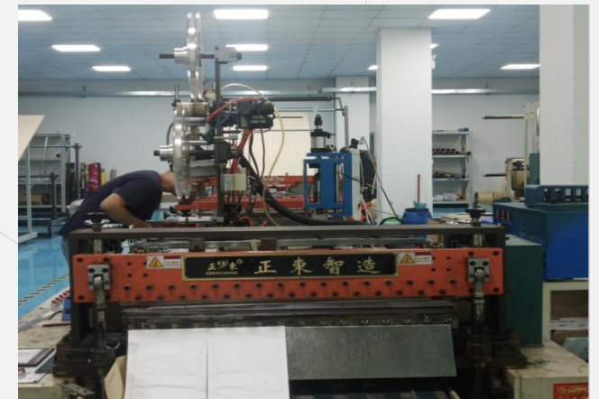
Cutting Into Bag Machine
